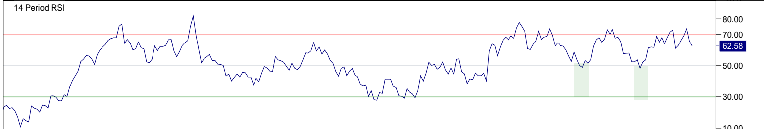
14 Period RSI
