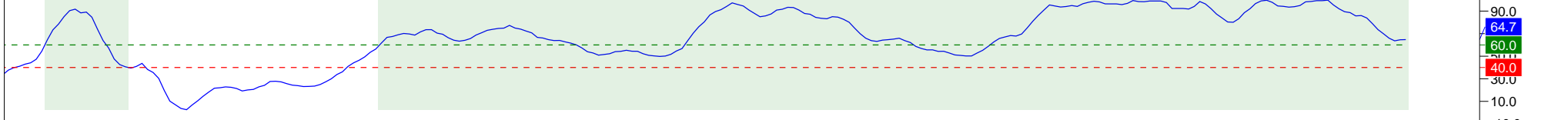
14 Period RSI
