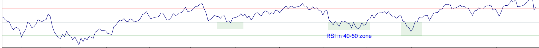
14 Period RSI
