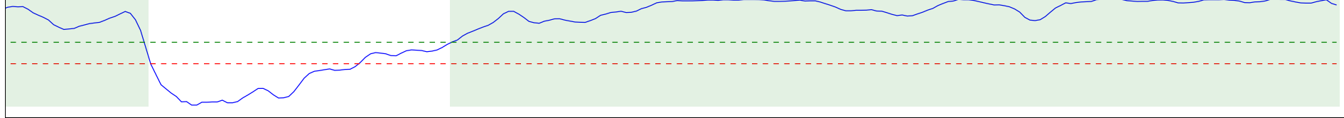
14 Period RSI
