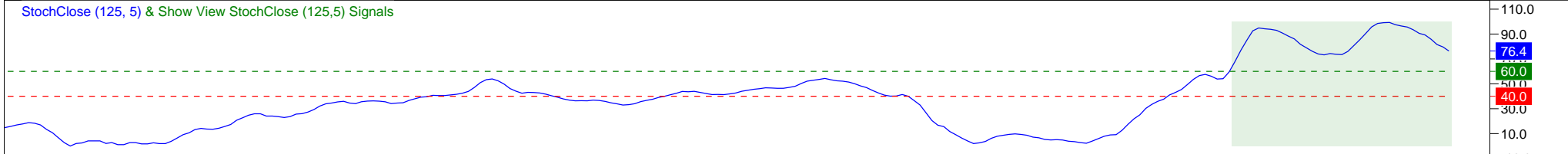
14 Period RSI
