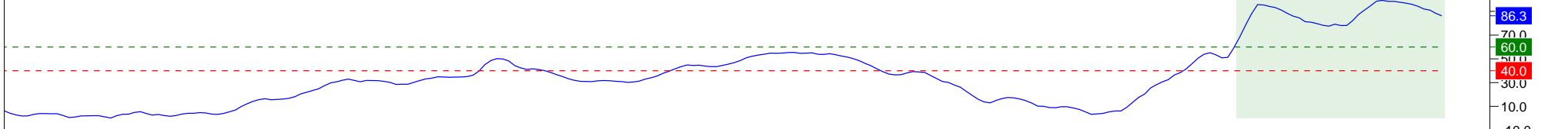
14 Period RSI
