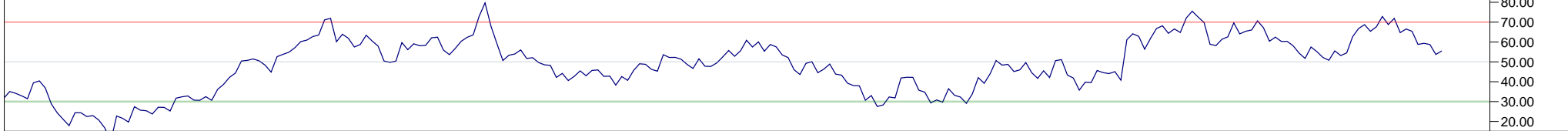
14 Period RSI
