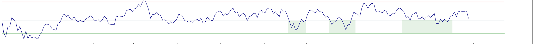
14 Period RSI
