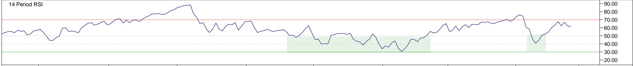
14 Period RSI
