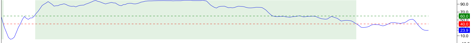
14 Period RSI
