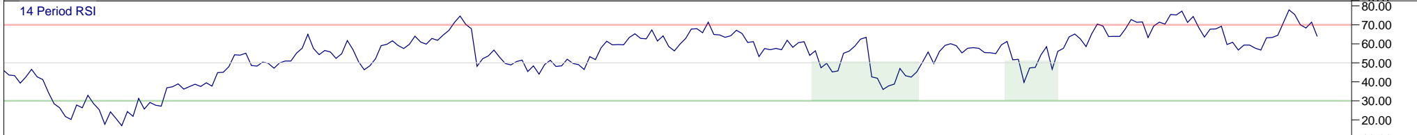
14 Period RSI
