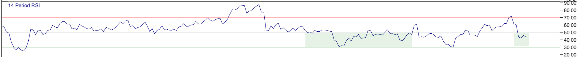
14 Period RSI
