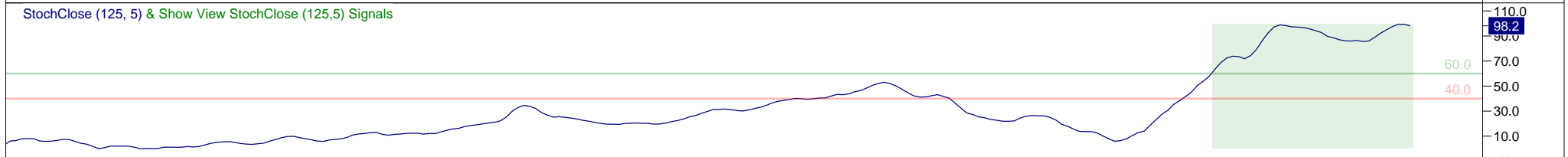
14 Period RSI
