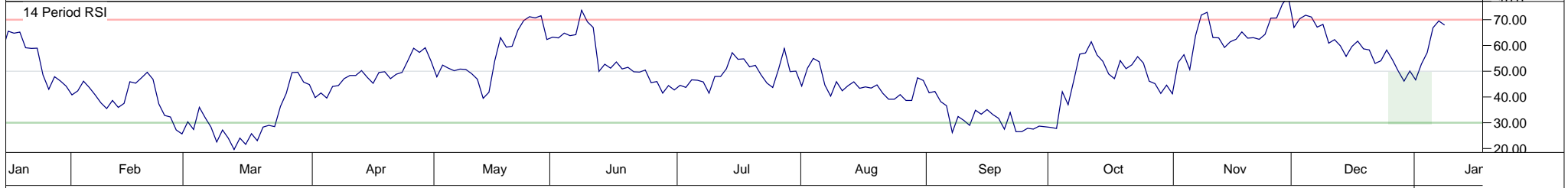
14 Period RSI
