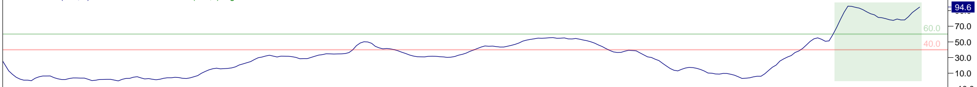
14 Period RSI
