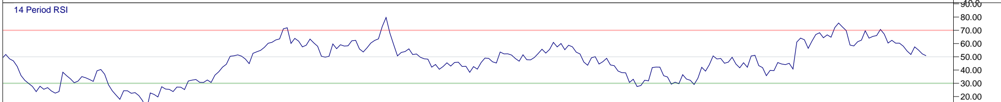
14 Period RSI
