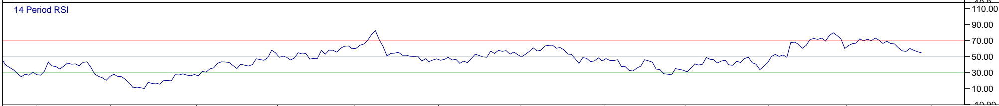
14 Period RSI
