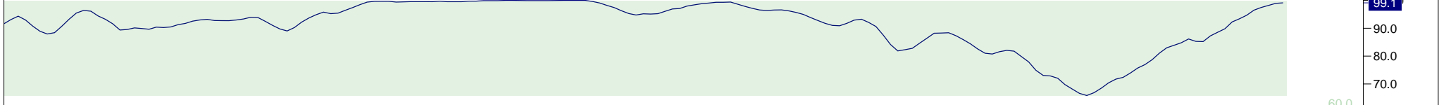
14 Period RSI
