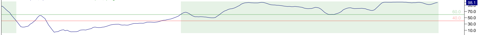
14 Period RSI
