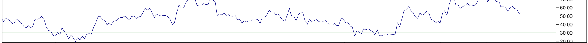
14 Period RSI
