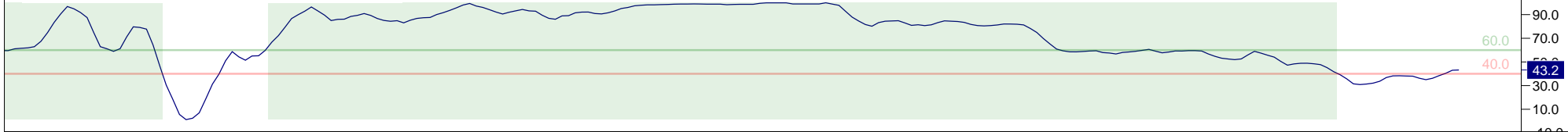
14 Period RSI
