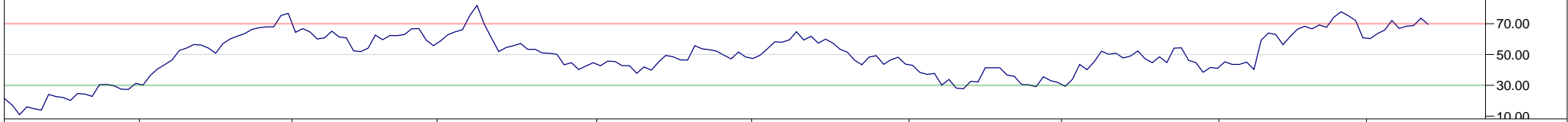
14 Period RSI
