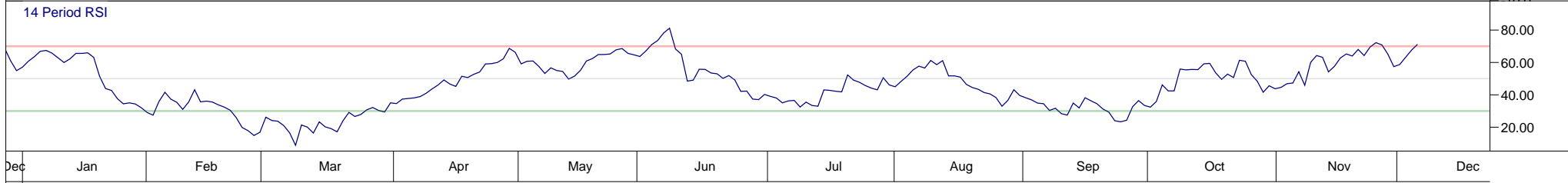
14 Period RSI
