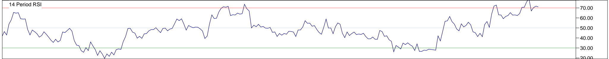
14 Period RSI
