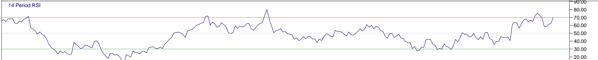
14 Period RSI
