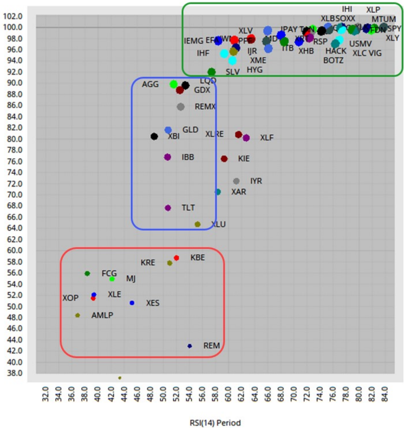
Stoch 125 (Closing Prices) 5-day SMA
