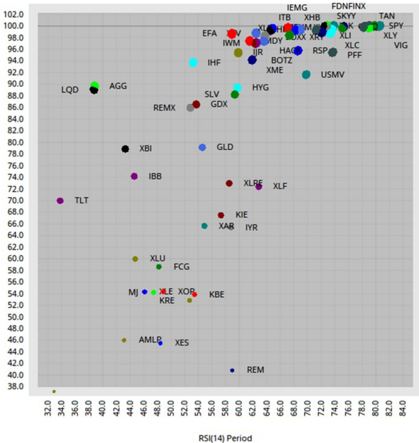
Stoch 125 (Closing Prices) 5-day SMA
