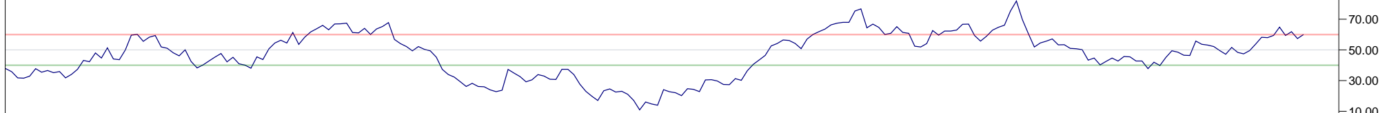
14 Period RSI
