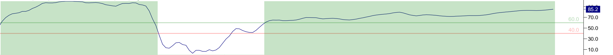
14 Period RSI
