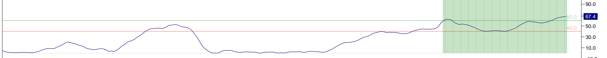
14 Period RSI
