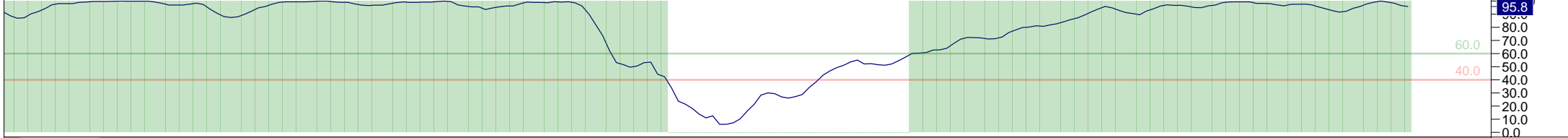
14 Period RSI
