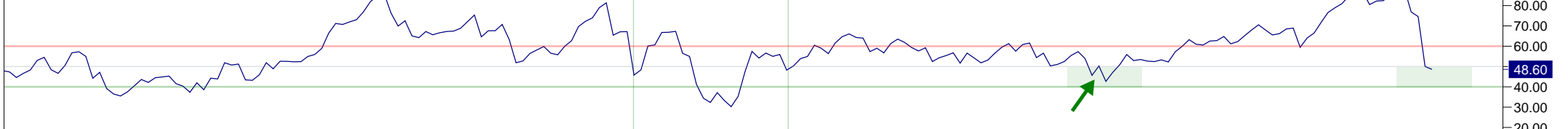
14 Period RSI
