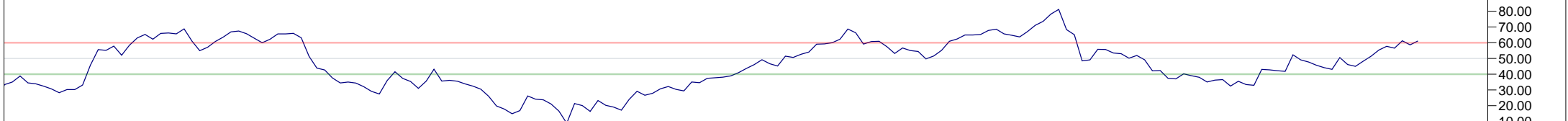
14 Period RSI
