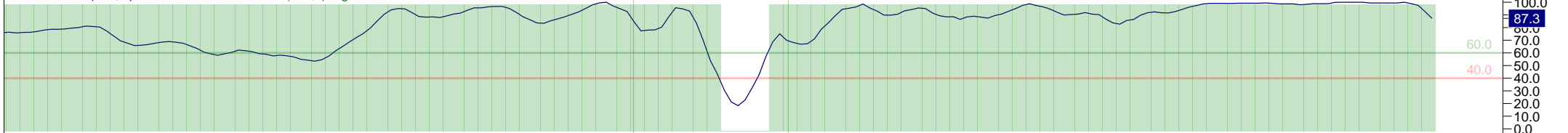
14 Period RSI
