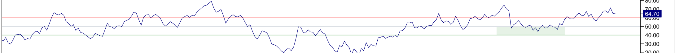
14 Period RSI
