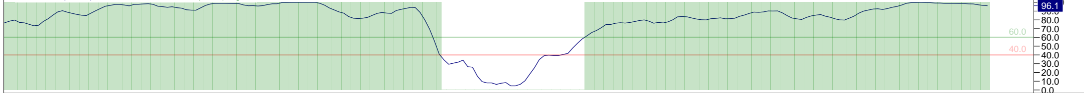
14 Period RSI
