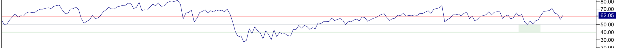
14 Period RSI
