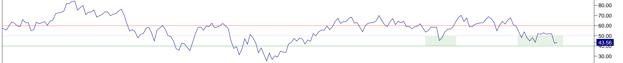
14 Period RSI
