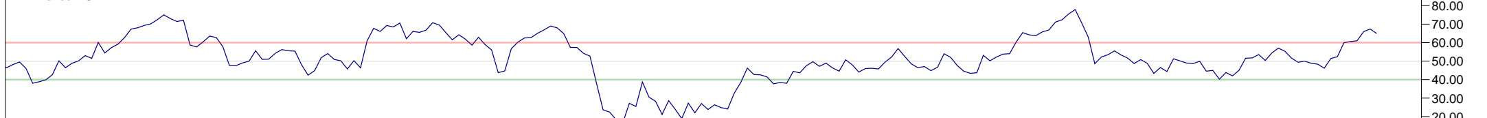
14 Period RSI
