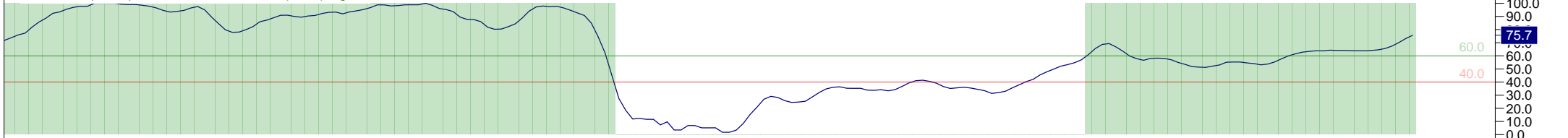
14 Period RSI
