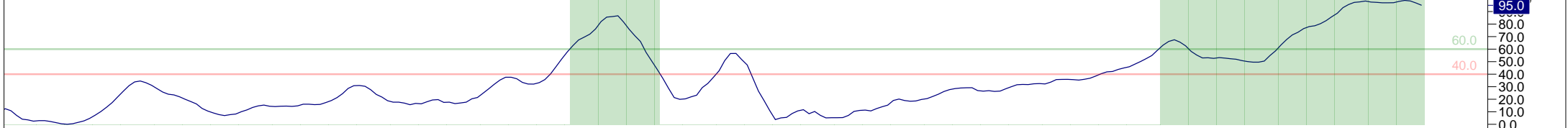
14 Period RSI
