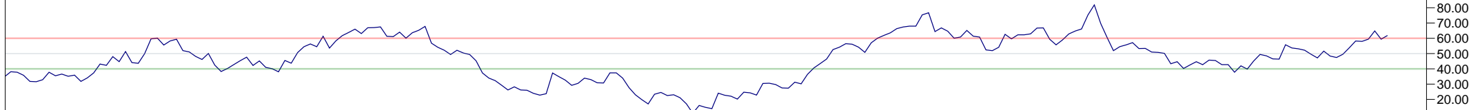
14 Period RSI
