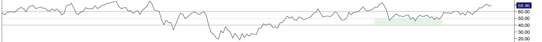
14 Period RSI
