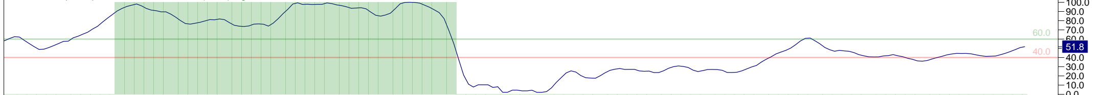
14 Period RSI
