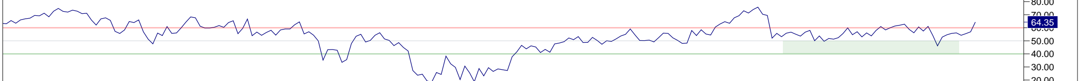
14 Period RSI
