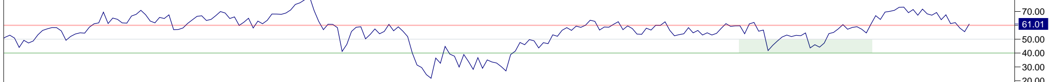
14 Period RSI
