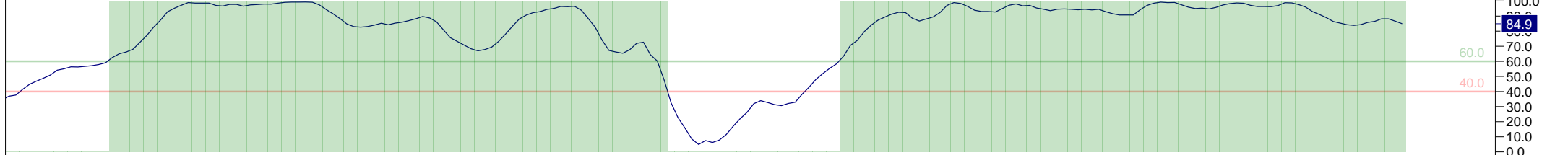
14 Period RSI
