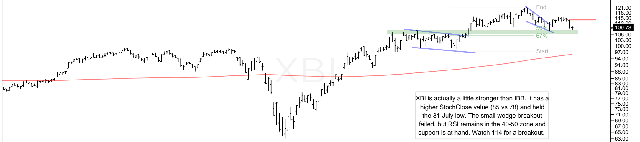
StochClose (125, 5) & Show View StochClose (125,5) Signals
