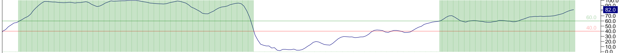
14 Period RSI
