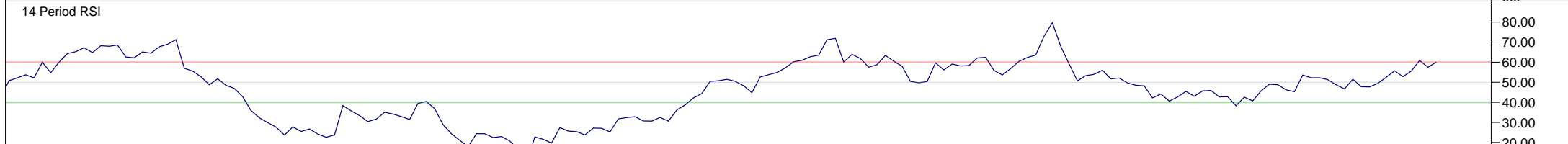
14 Period RSI
