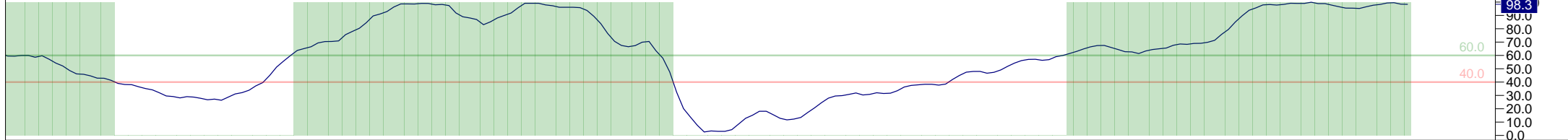
14 Period RSI
