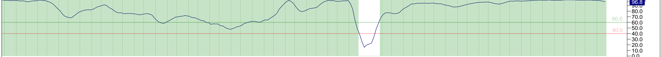
14 Period RSI
