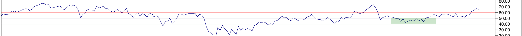
14 Period RSI
