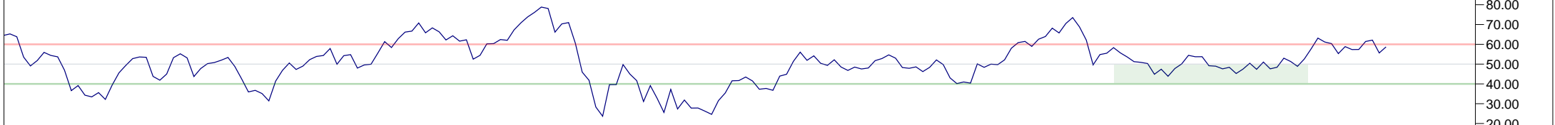
14 Period RSI
