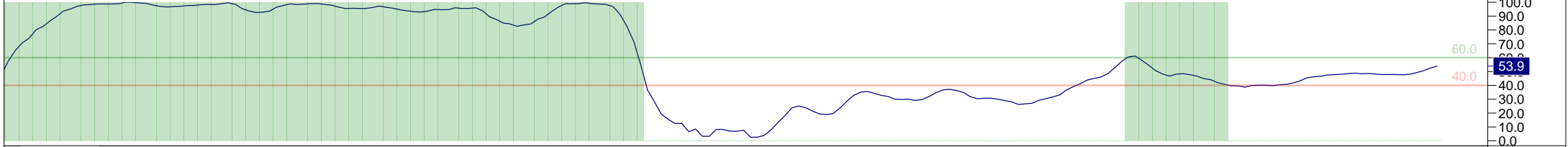
14 Period RSI
