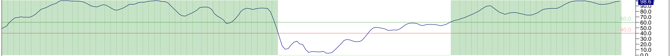
14 Period RSI
