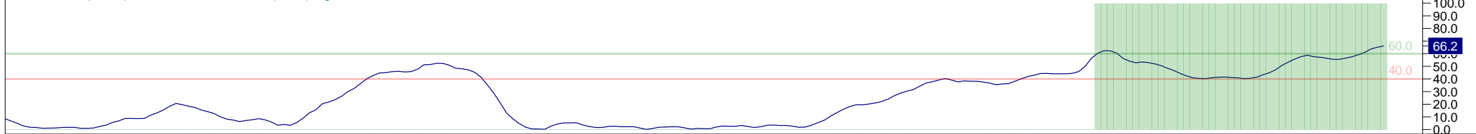
14 Period RSI
