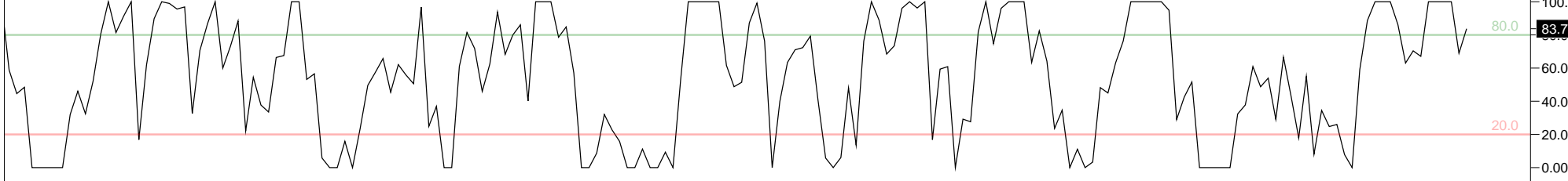
StochRSI
