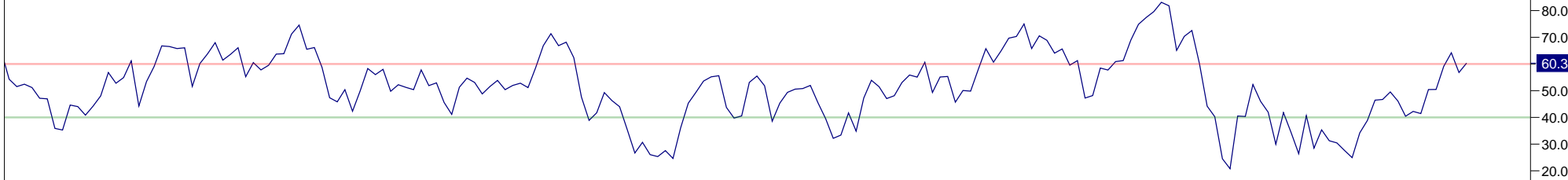
StochRSI
