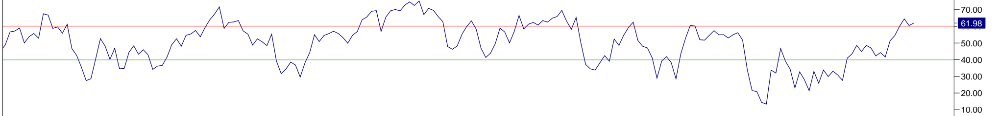
StochRSI
